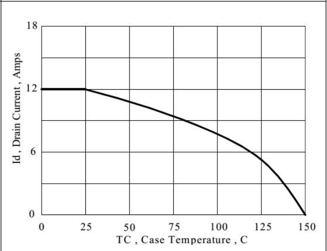
Figure 4. Maximum Drain Current with Case Temperature
