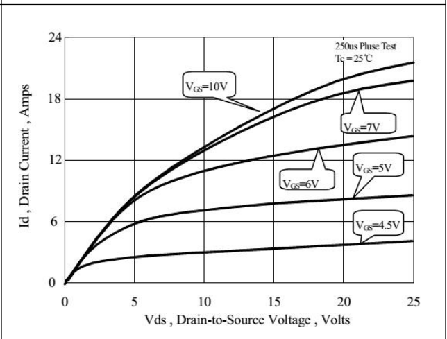
Figure 6. On-State Characteristics
